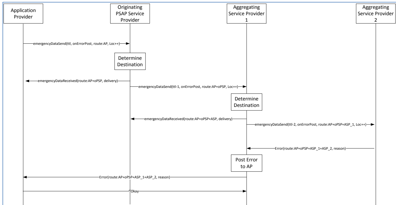
Figure 2 onErrorPost message flow
