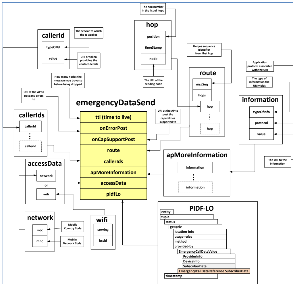
Figure 1 emergencyDataSend message structure
