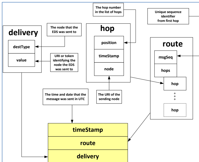
Figure 4 emergencyDataReceived message structure
