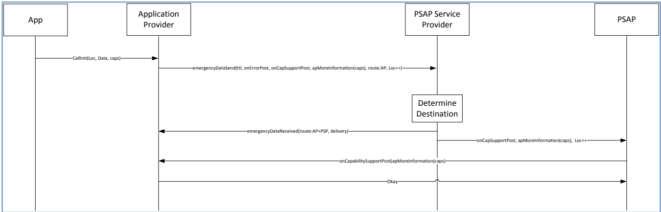
Figure 3 onCapSupportPost message sequence
